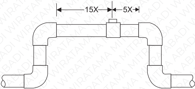
Two Elbows, In Plane
