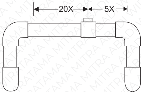
Two Elbows, Out Of Plane
