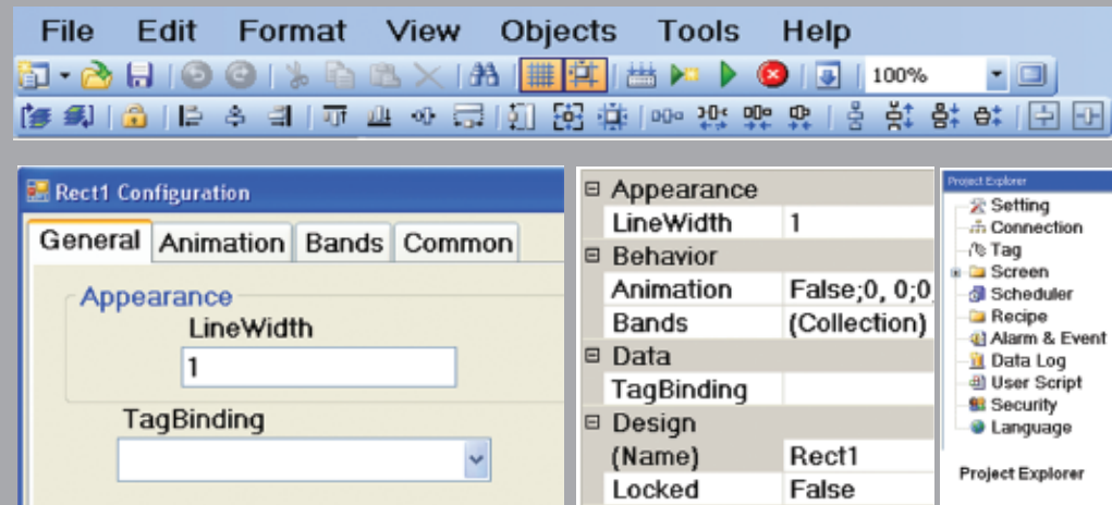
GUI Wizard
